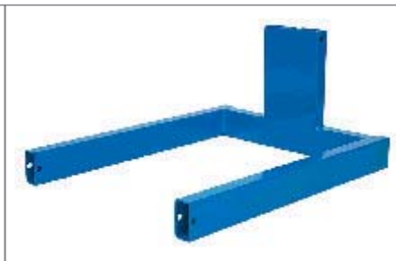
Standard Fork ◆ Load capacity 300 kg ◆ To lift construction parts ◆ Weight 14 kg ◆ Dimension: 600 x 700 mm
